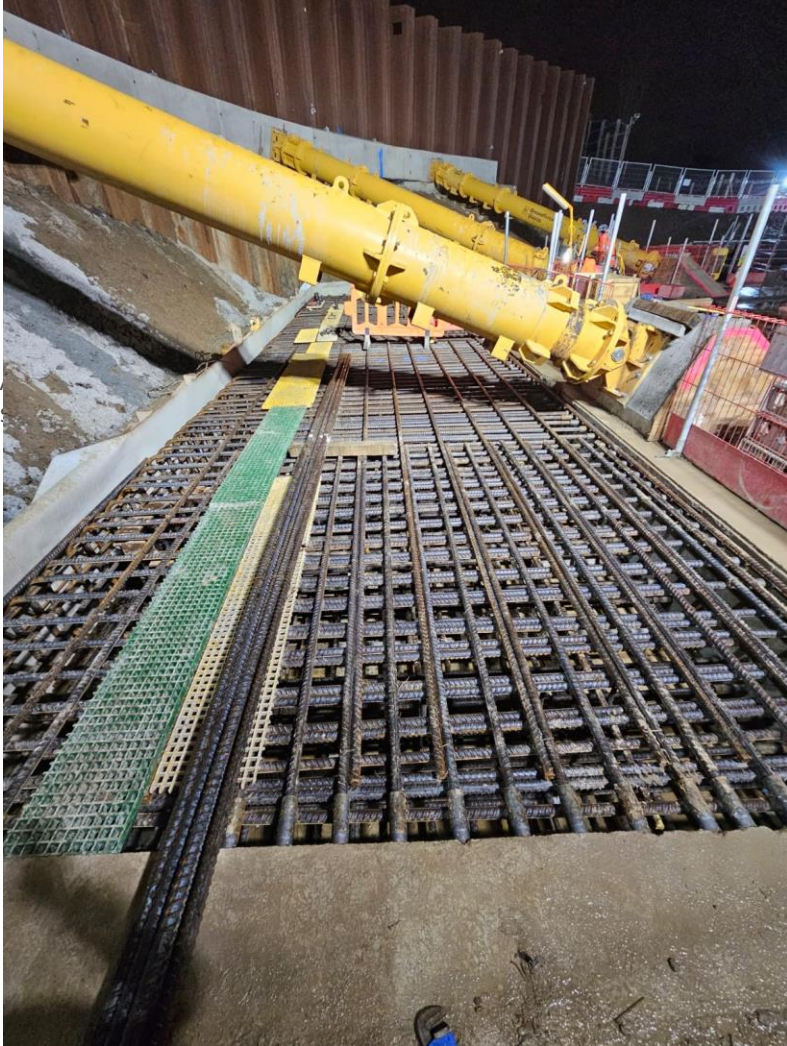
Headhouse base slab steel fixing
