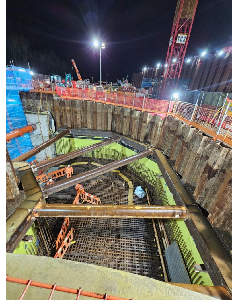
Ongoing ventilation basement construction
