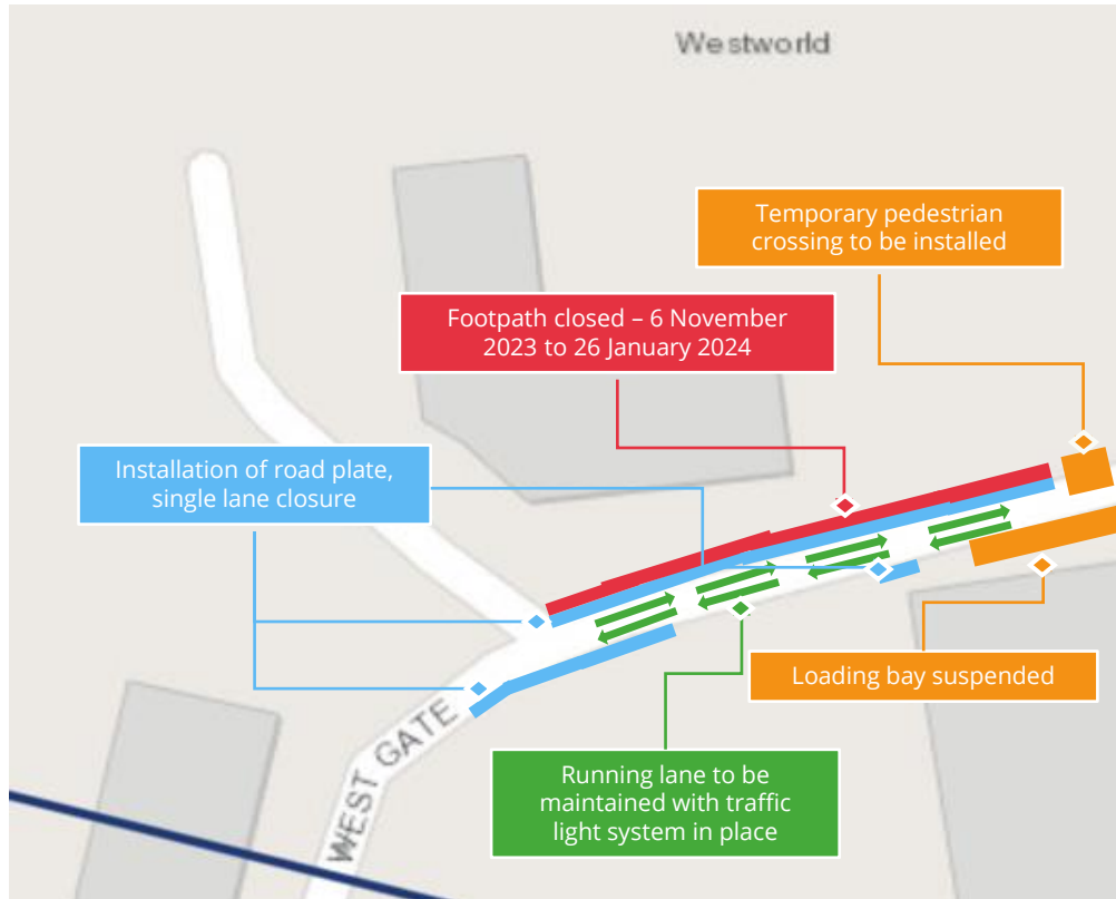
Phase One B - 20 November 2023 to 26 January 2024. Road plate installation
